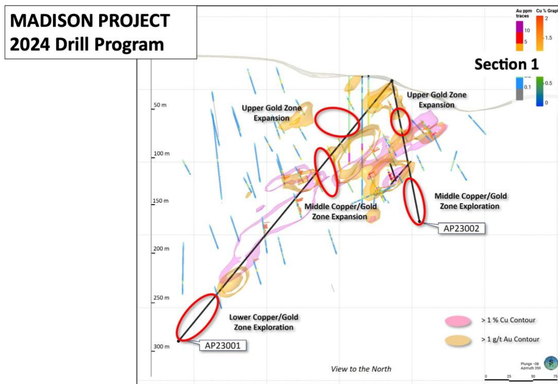
Figure 2. 2024 Madison Drilling. Section 1, Mineral inventory expansion and definition.
