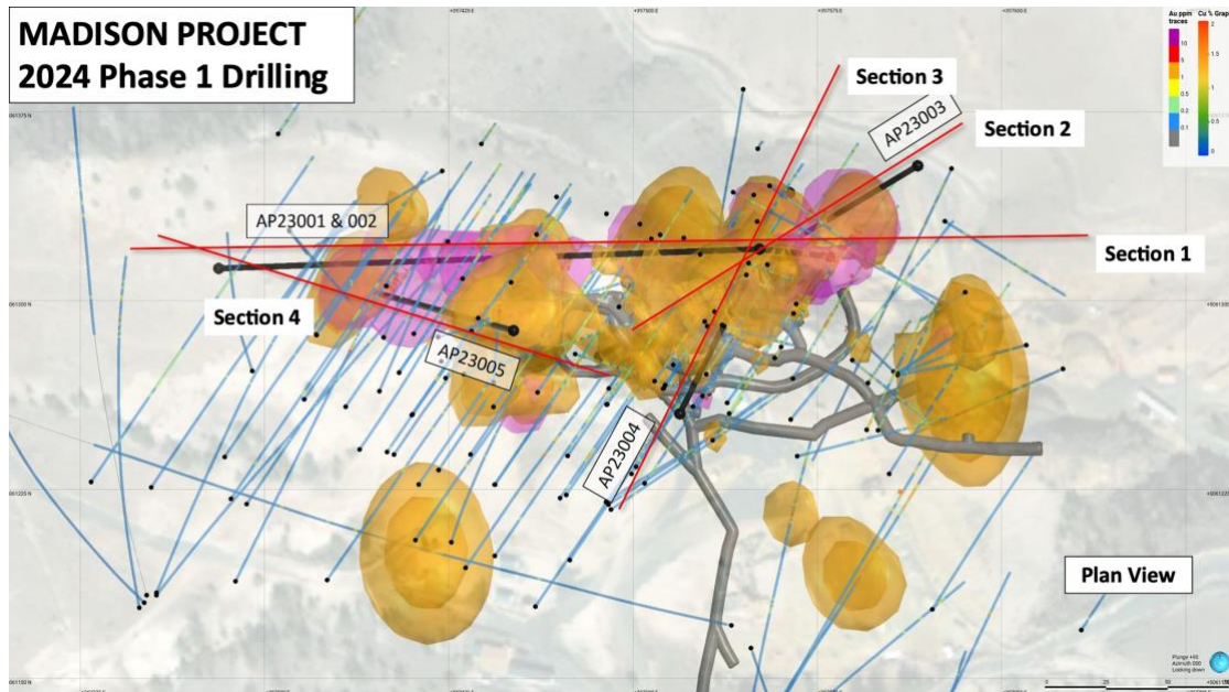
Figure 1. 2024 Madison Drilling. Plan map showing drill site locations.
