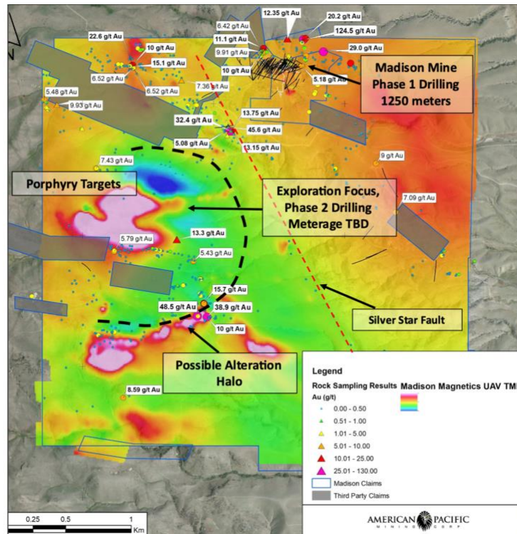
Figure 3. Madison Property magnetic data with rock chip gold values and exploration focus areas.
